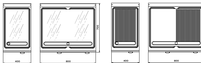
PIASTRA CROMATA / CHROMED PLATE
